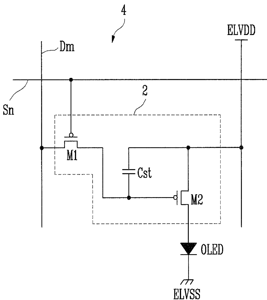
FIG. 1 (PRIOR ART)
